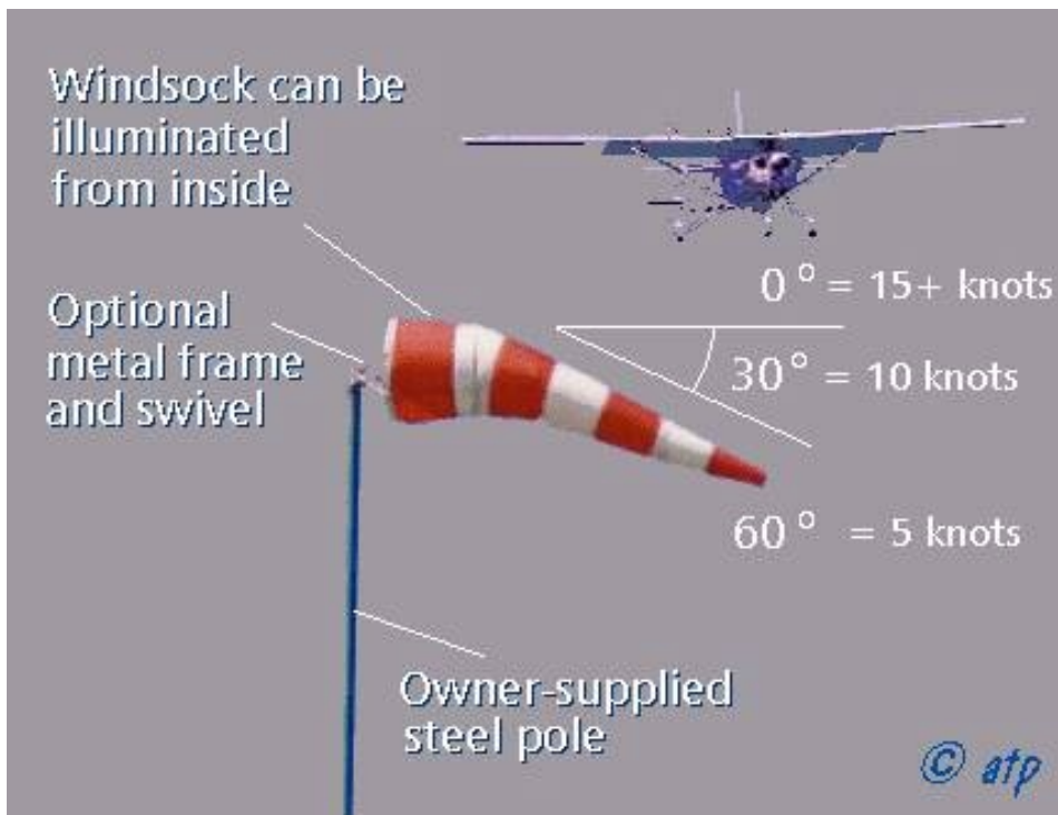
Fig 6-11 Airport Windsock
