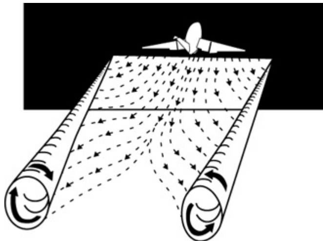
Figure 6-17.—Vortex generation.
