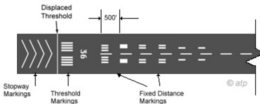
Figure 6-3.—Selected runway markings.
